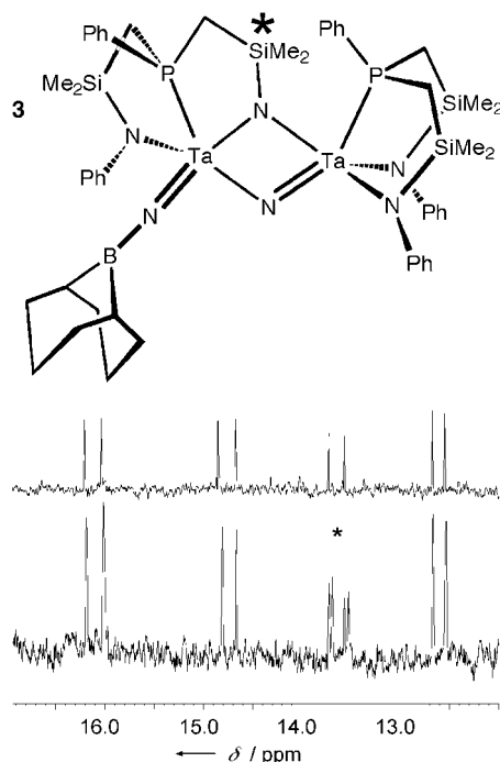
Figure 3. 29 Si-DEPT NMR spectra of complex 3 (top) and the isotopomer 15 N 2 - 3 (bottom). Additional splitting in the peak at δ = 13.64 ppm (*) is a result of 15 N coupling ( I = 1/2, 1 J N,Si = 3.2 Hz).
